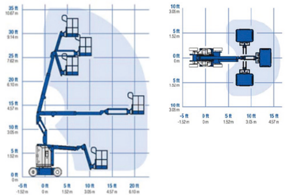
RANGE OF MOTION Z 30 /20N RJ
